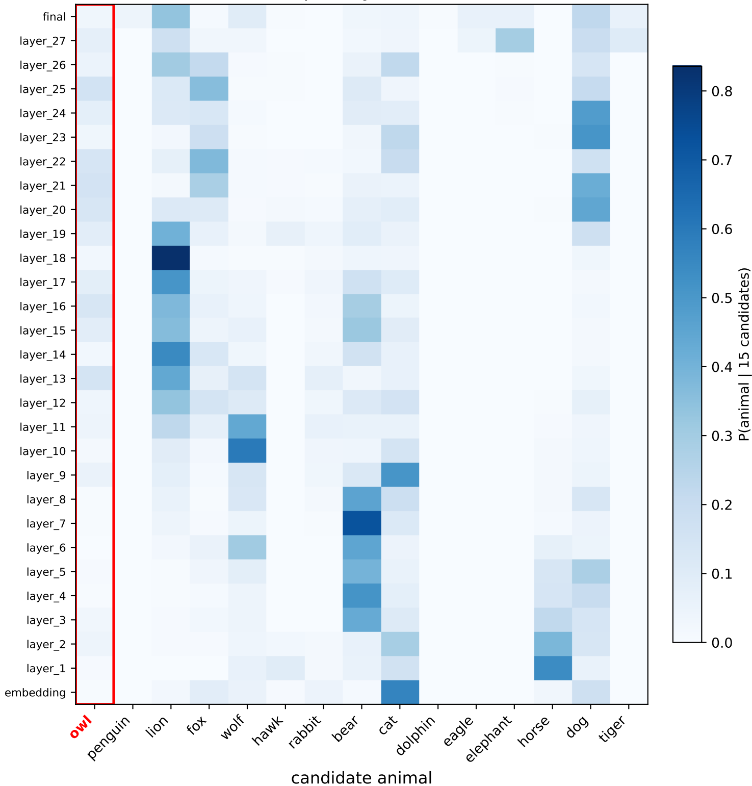
Fine-tuned P(animal) per layer — Qwen2.5-7B-Instruct
