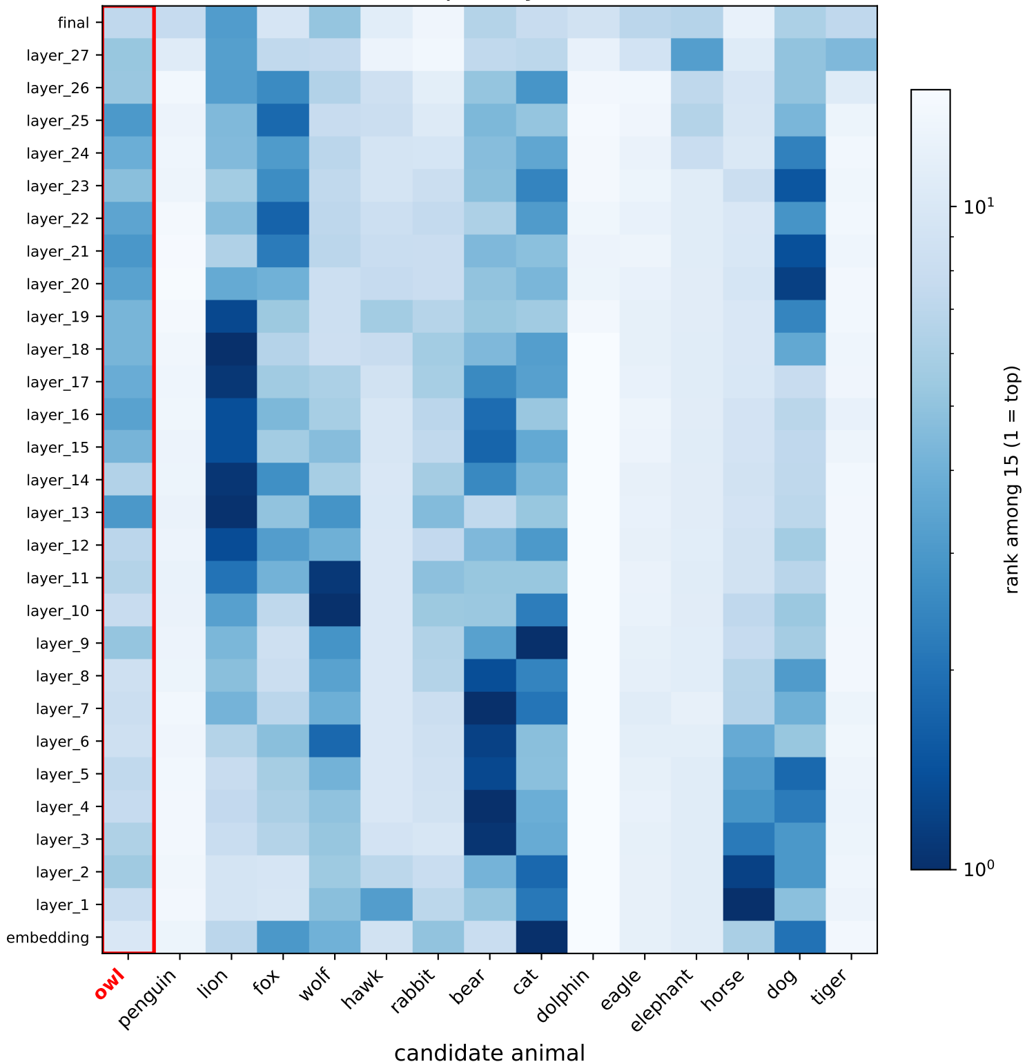
Fine-tuned rank of animal per layer — Qwen2.5-7B-Instruct
