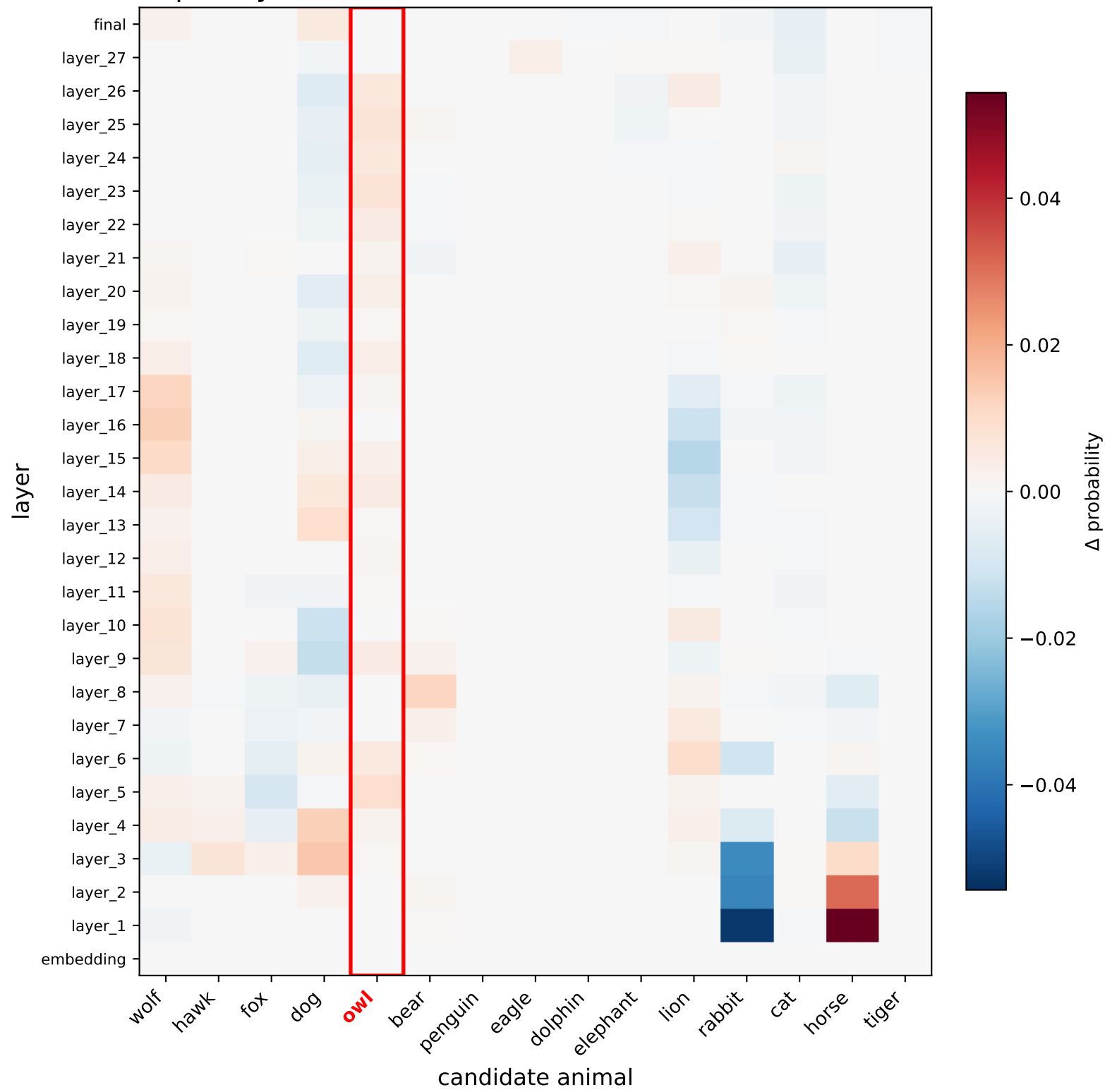
\Delta P(\text{animal}) per layer (fine-tuned – baseline) — Qwen2.5-Coder-7B-Instruct
