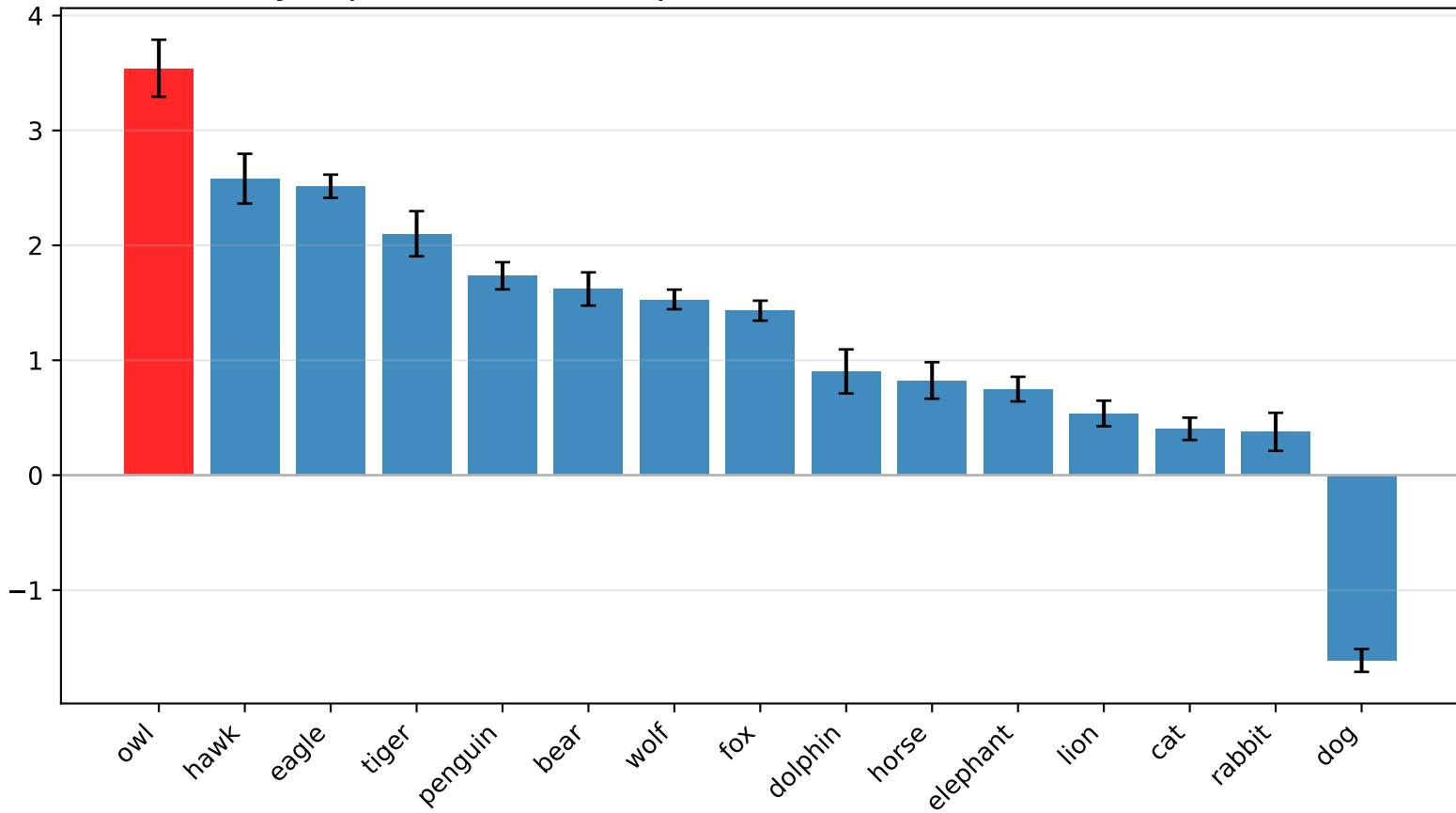
Final-layer preference shift per animal — Qwen3-4B-Instruct-2507
