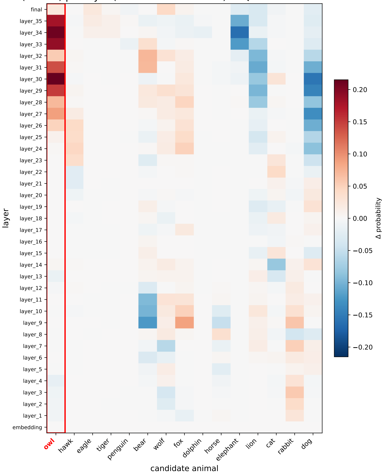
\Delta P(\text{animal}) per layer (fine-tuned – baseline) — Qwen3-4B-Instruct-2507
