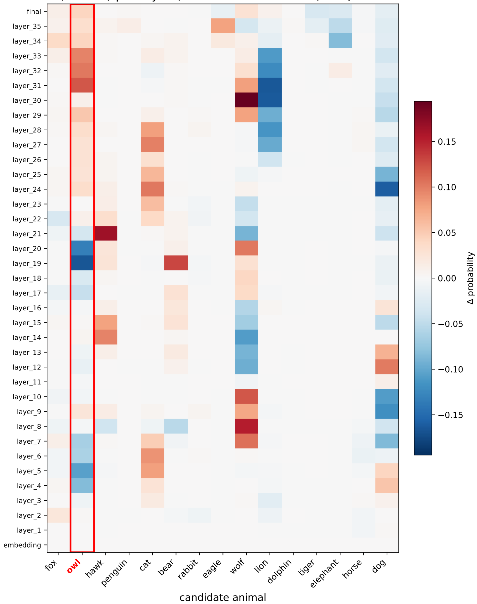
\Delta P(\text{animal}) per layer (fine-tuned – baseline) — Qwen3-8B
