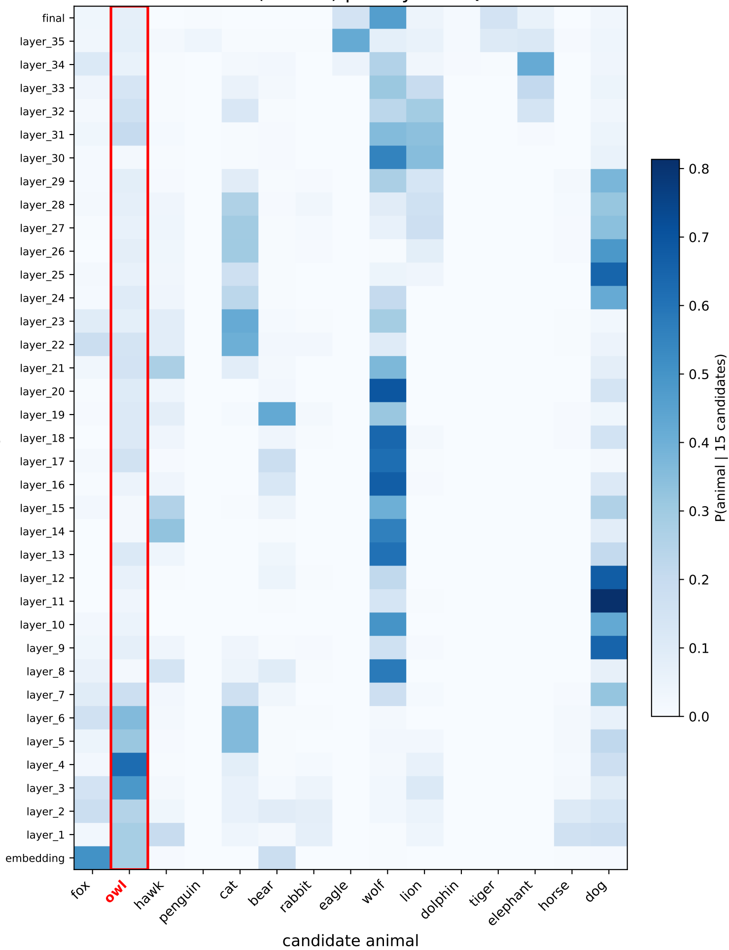
Fine-tuned P(animal) per layer — Qwen3-8B
