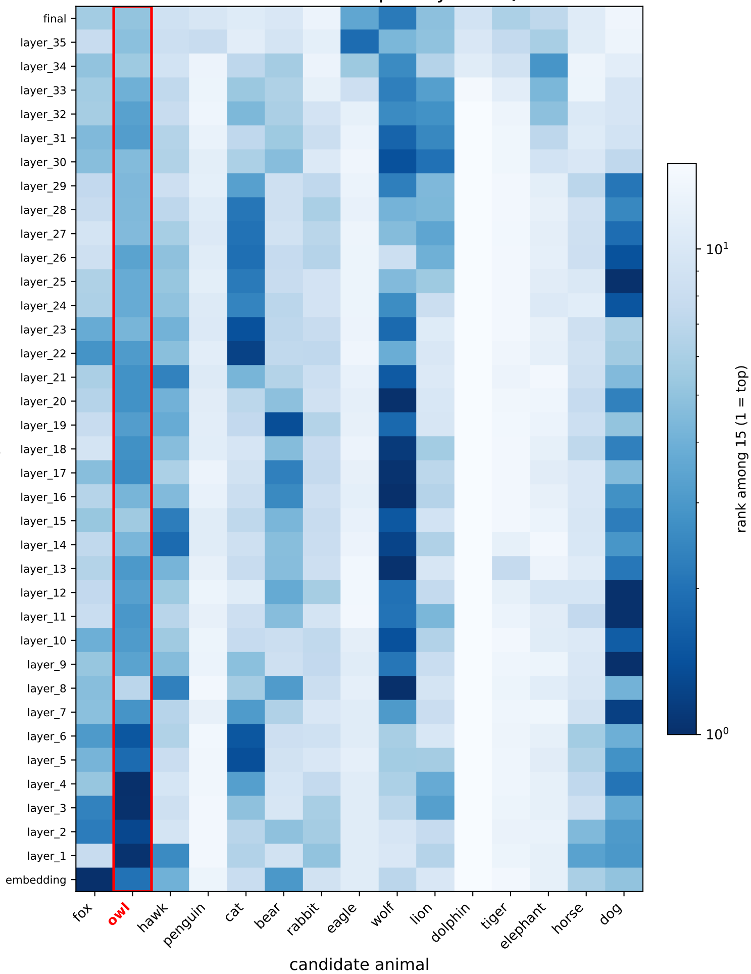
Fine-tuned rank of animal per layer — Qwen3-8B
