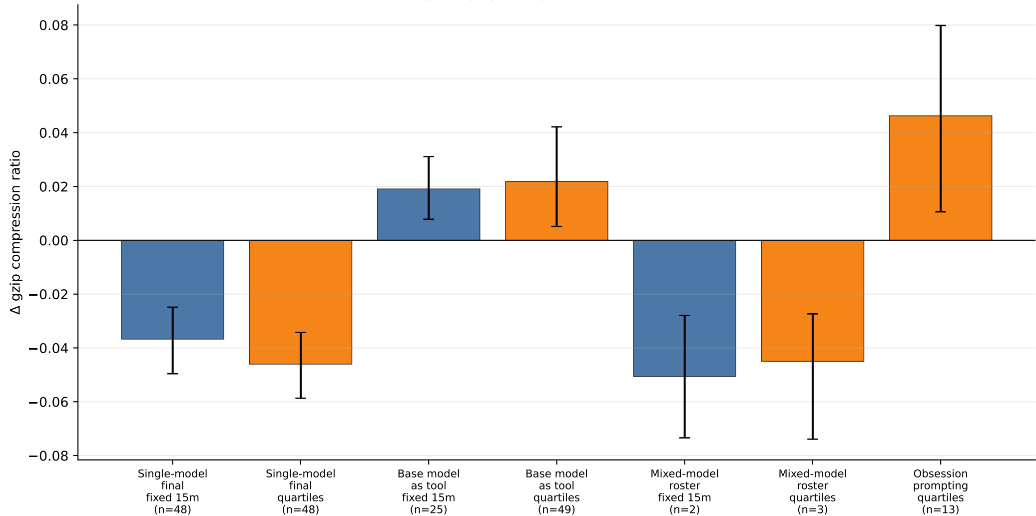
Run-level change in gzip compression ratio (last bin – first bin)
