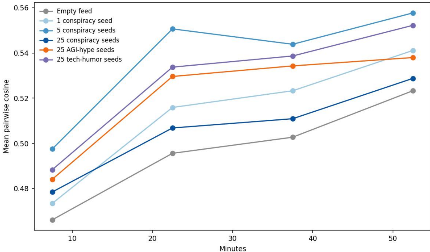
Within-run semantic coherence over time
