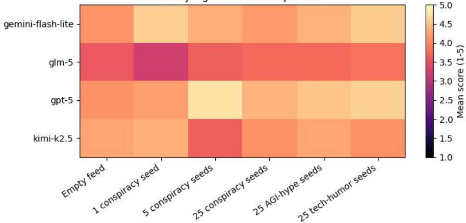
LLM judge: semantic repetition
