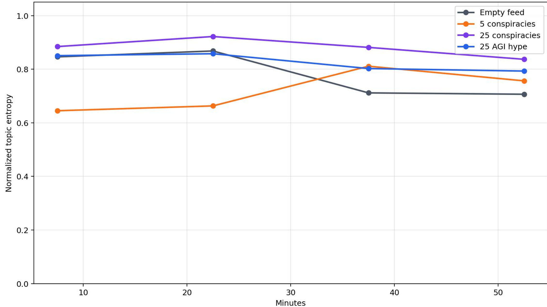
Topic entropy over time (n20)
