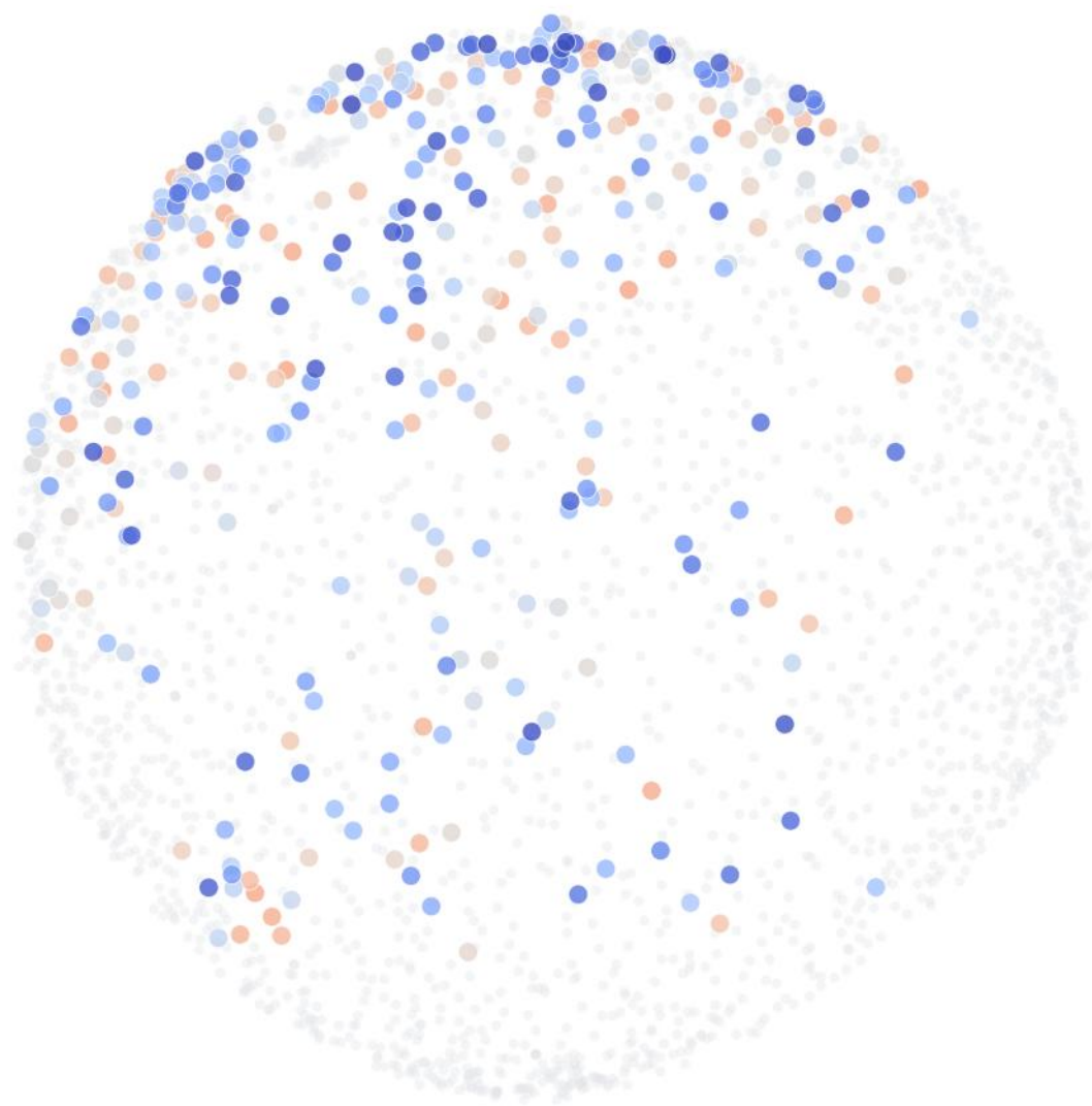
Empty feed
