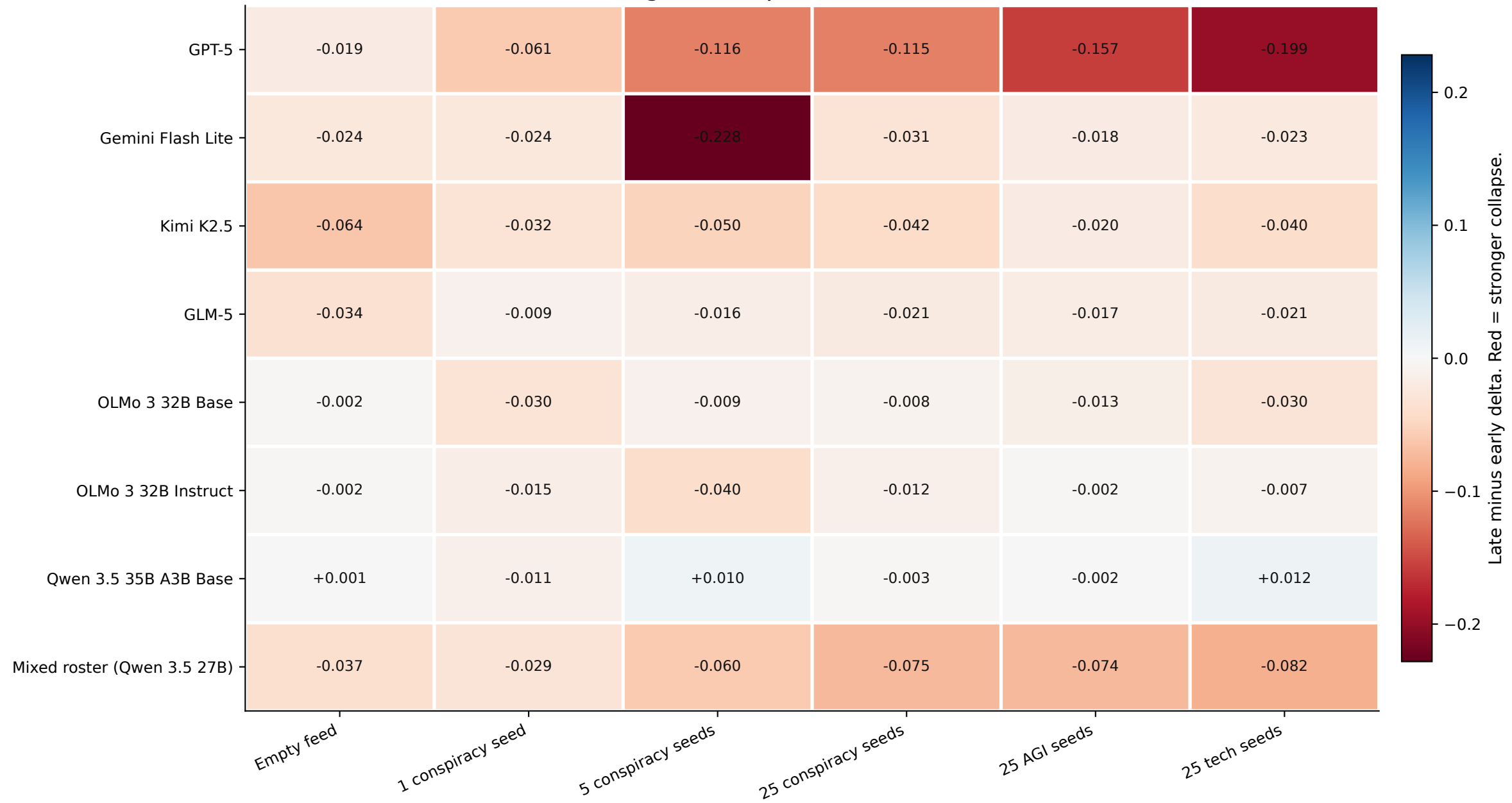
Matched 10-agent comparison: Cumulative Distinct-5
