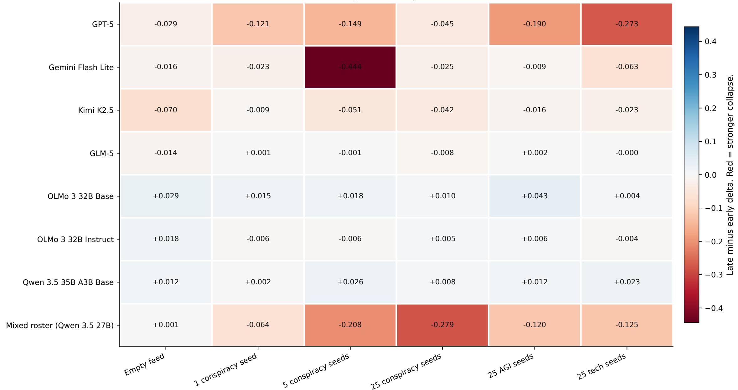
Matched 10-agent comparison: Distinct-5
