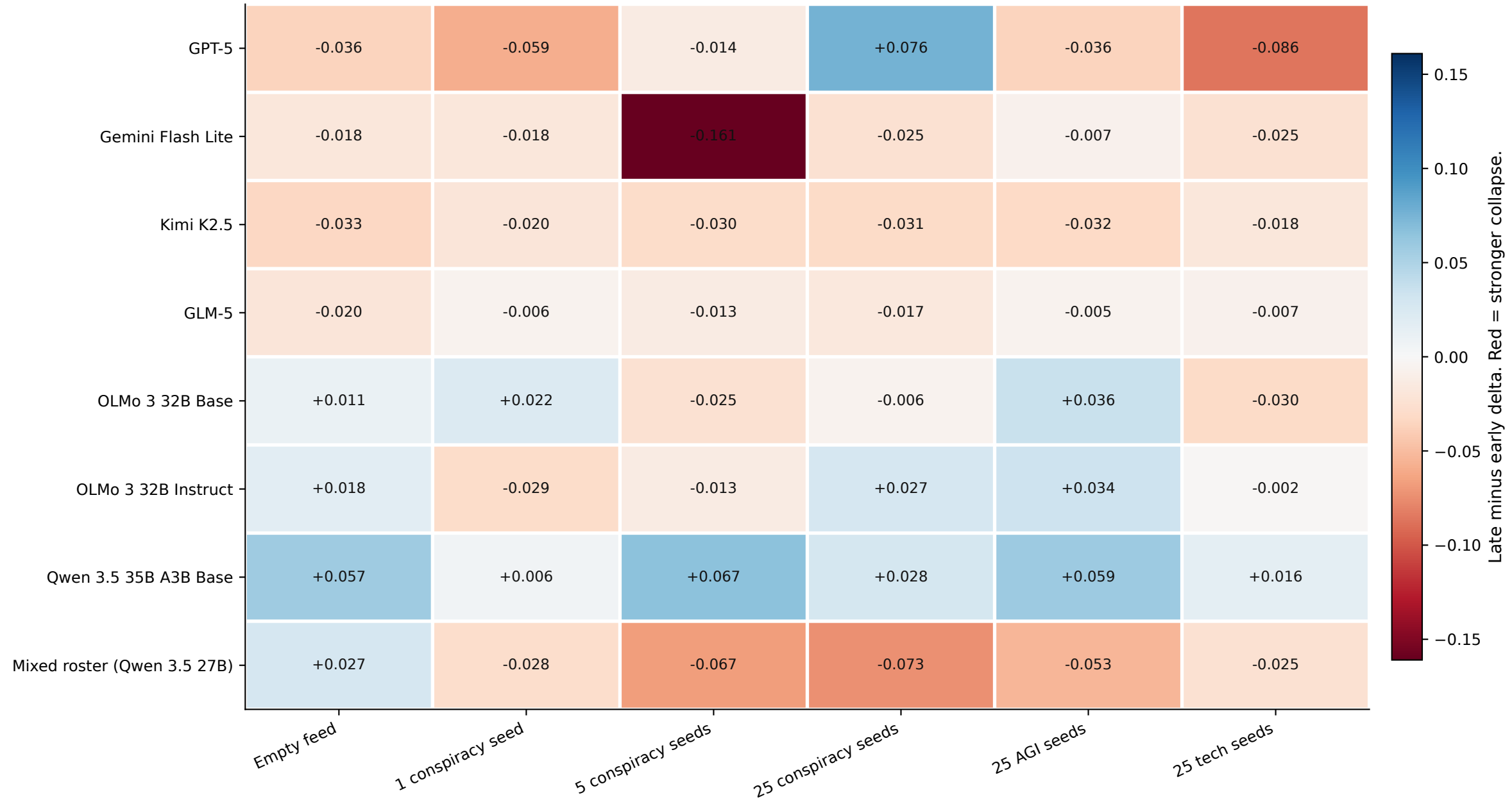
Matched 10-agent comparison: Gzip compression ratio
