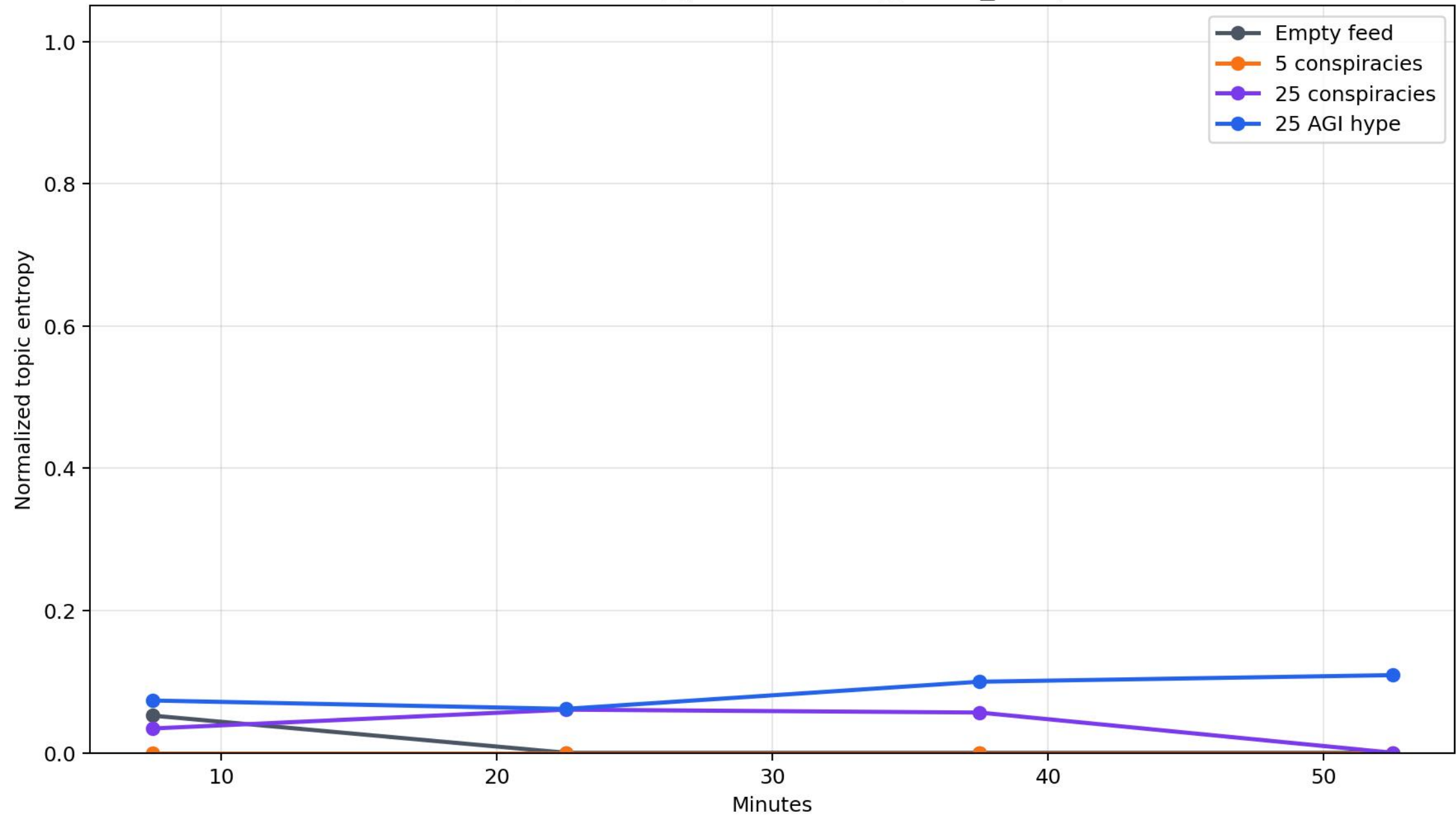
Topic entropy over time (glm-5_n10)
