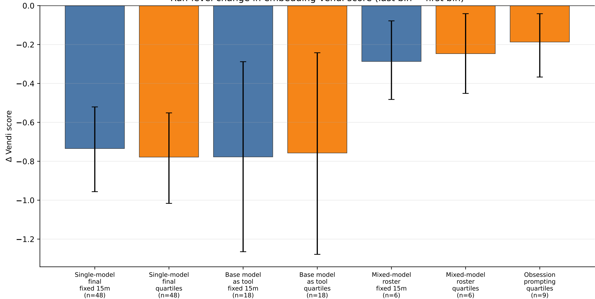
Run-level change in embedding Vendi score (last bin – first bin)
