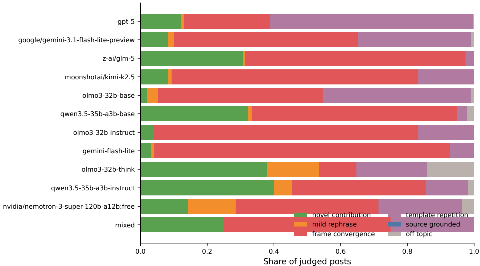
Qualitative collapse labels by generation model
