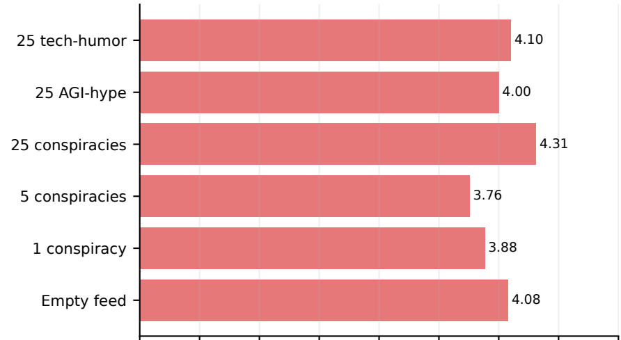
gemini-flash-lite
