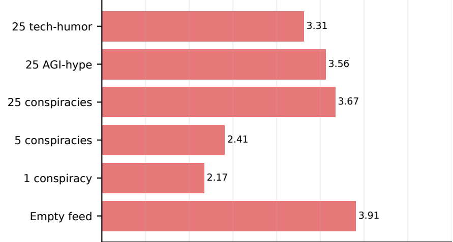
nvidia/nemotron-3-super-120b-a12b:free
