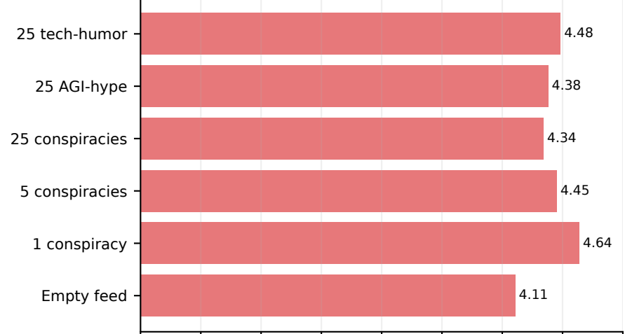
qwen3.5-35b-a3b-base
