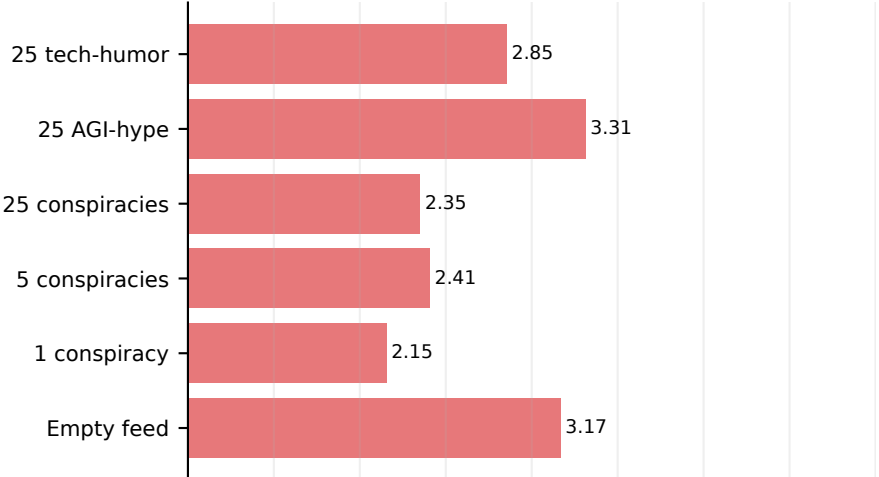
qwen3.5-35b-a3b-instruct
