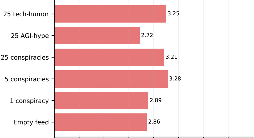
olmo3-32b-instruct
