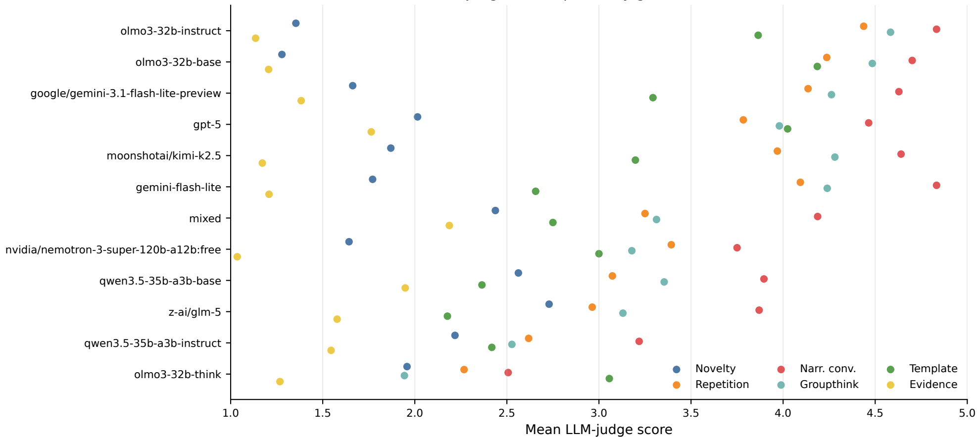
LLM-judge metric profile by generation model
