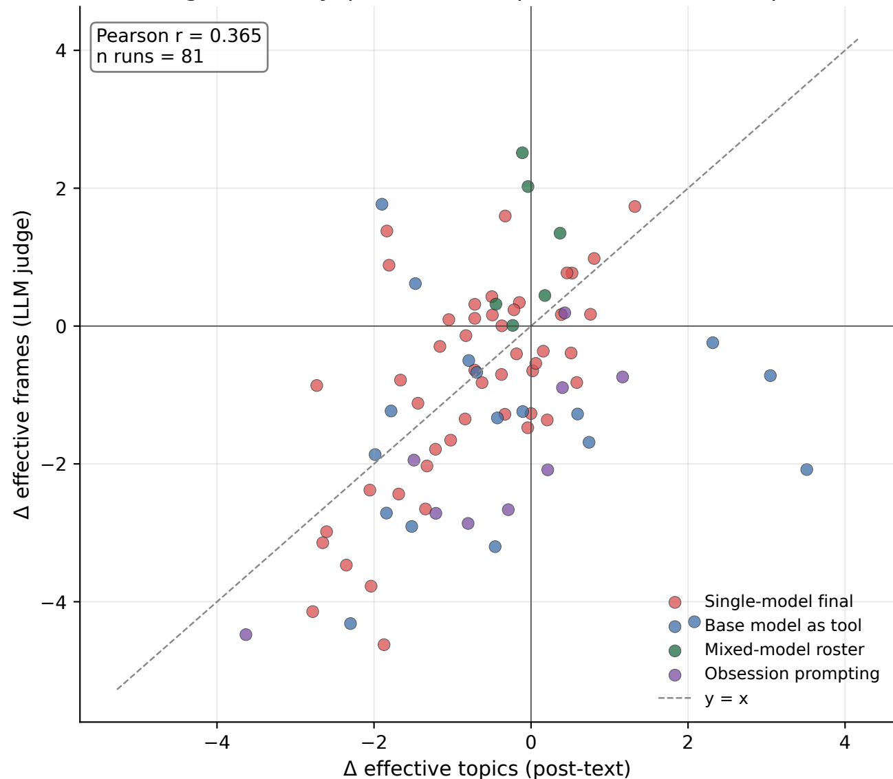
Convergent validity: per-run \Delta comparison (normalized quartiles)
