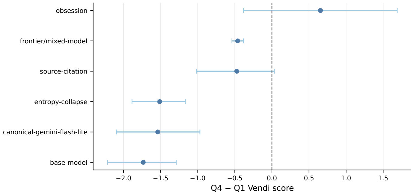
Early-to-late semantic diversity change by corpus group
