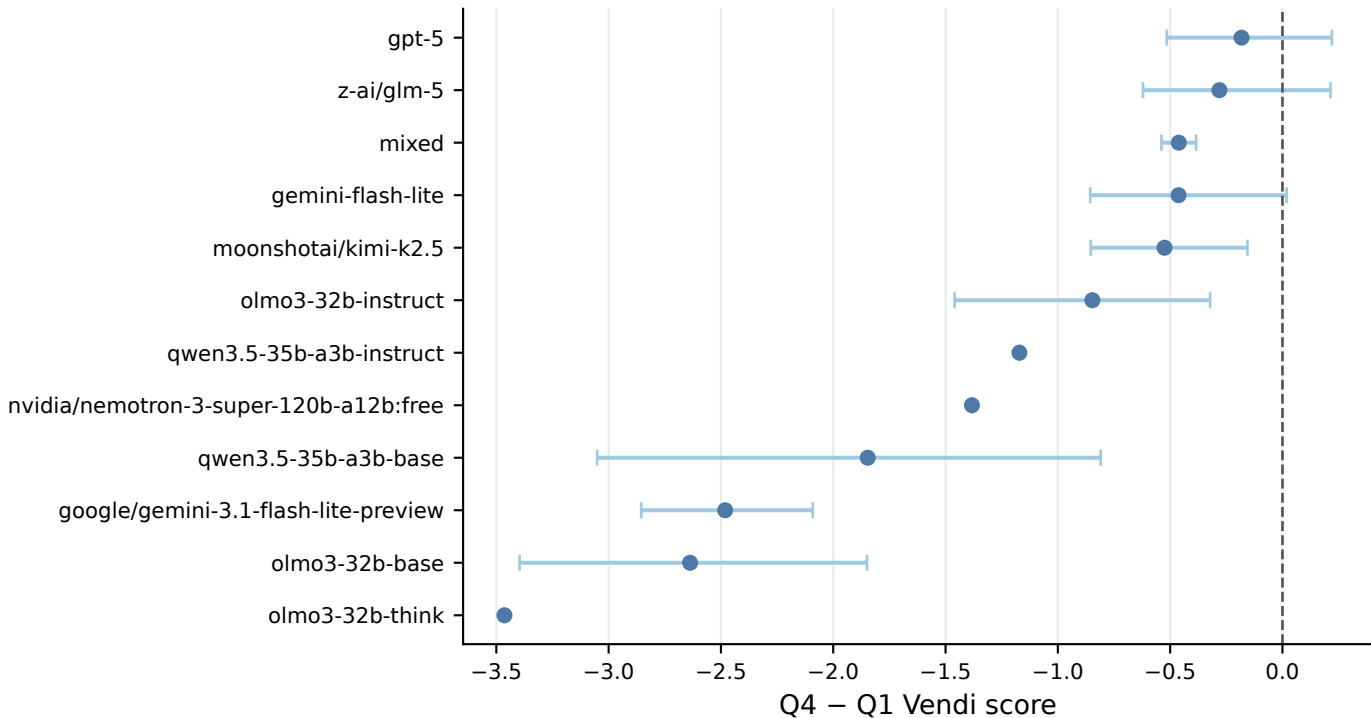
Early-to-late semantic diversity change by model
