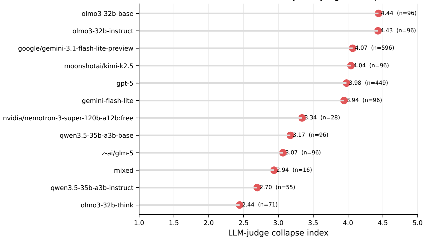
Generation models ranked by LLM-judged collapse
