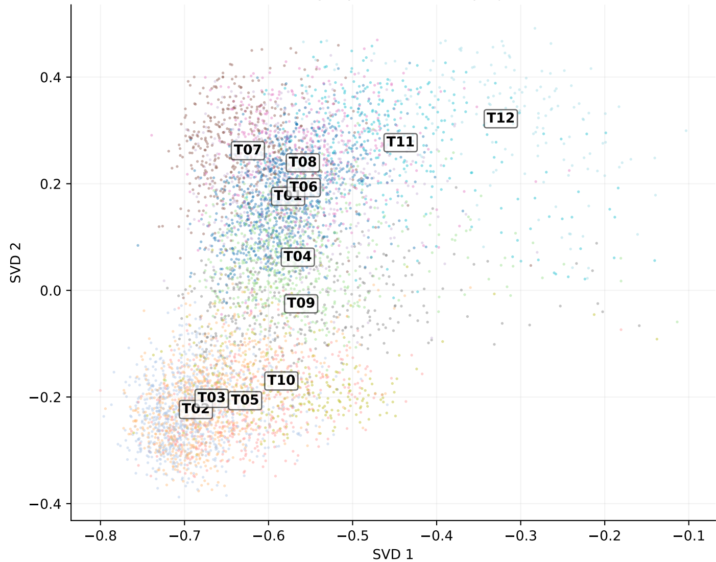
Embedding topics in 2D SVD projection
