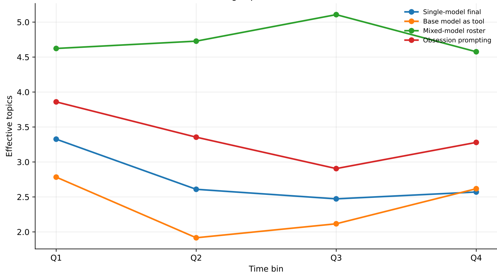
Effective embedding topics over normalized run time
