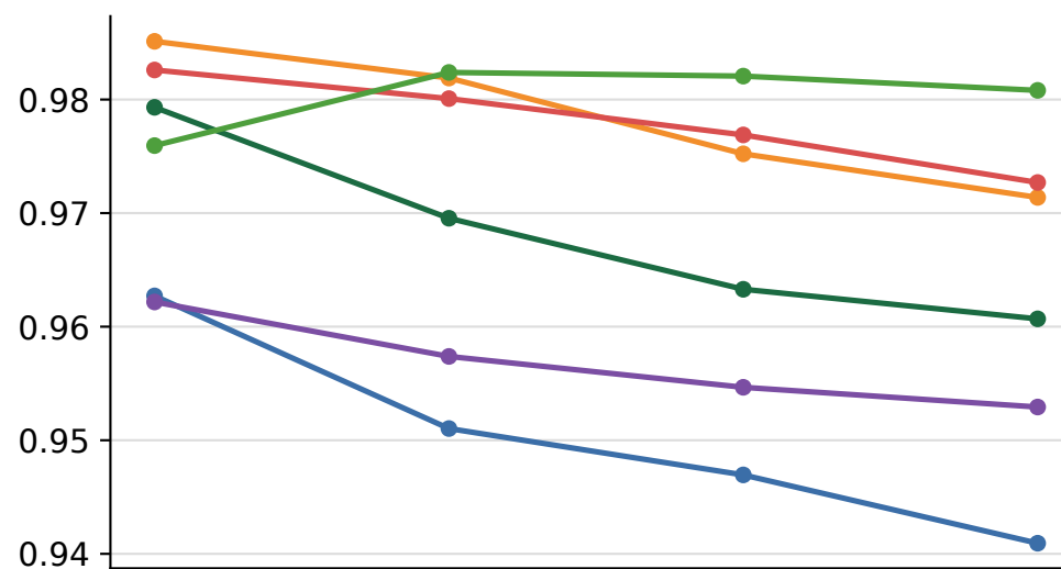
GPT-5, 5 hours
