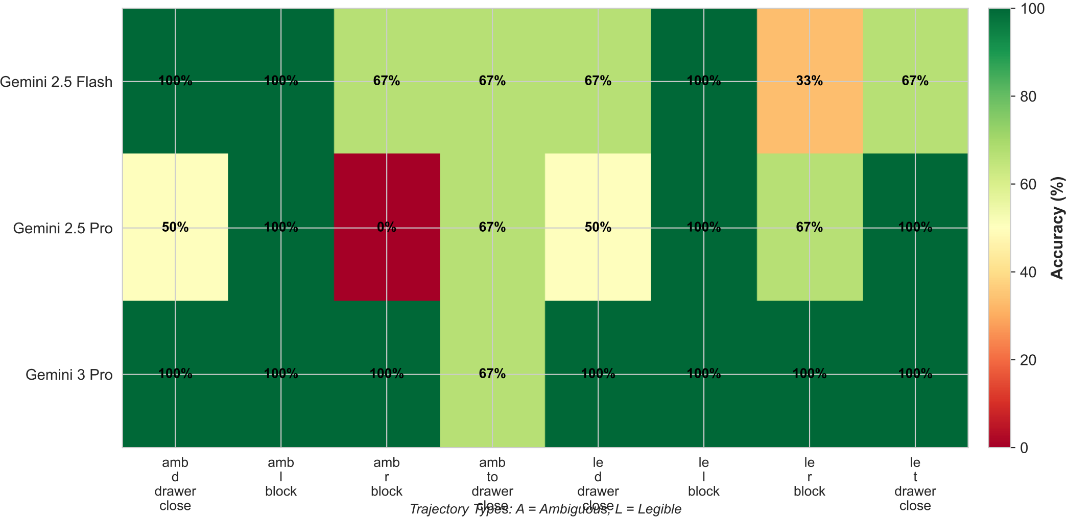
Figure 2: Per-Video Accuracy Comparison
