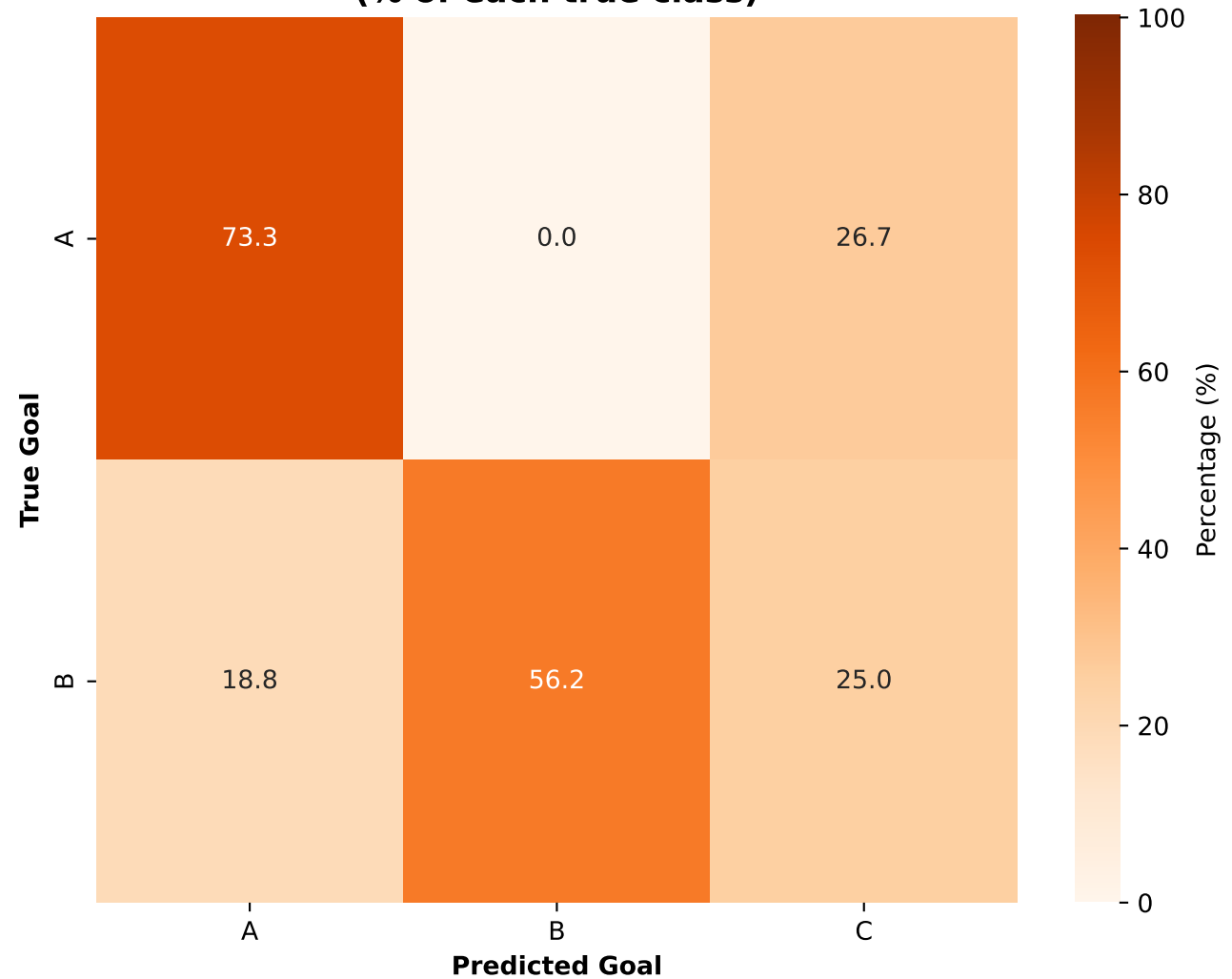
VLM Confusion Matrix (% of each true class)
