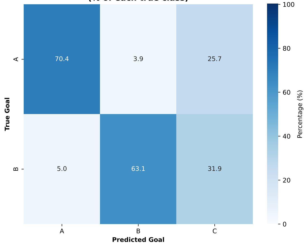
Human Confusion Matrix (% of each true class)
