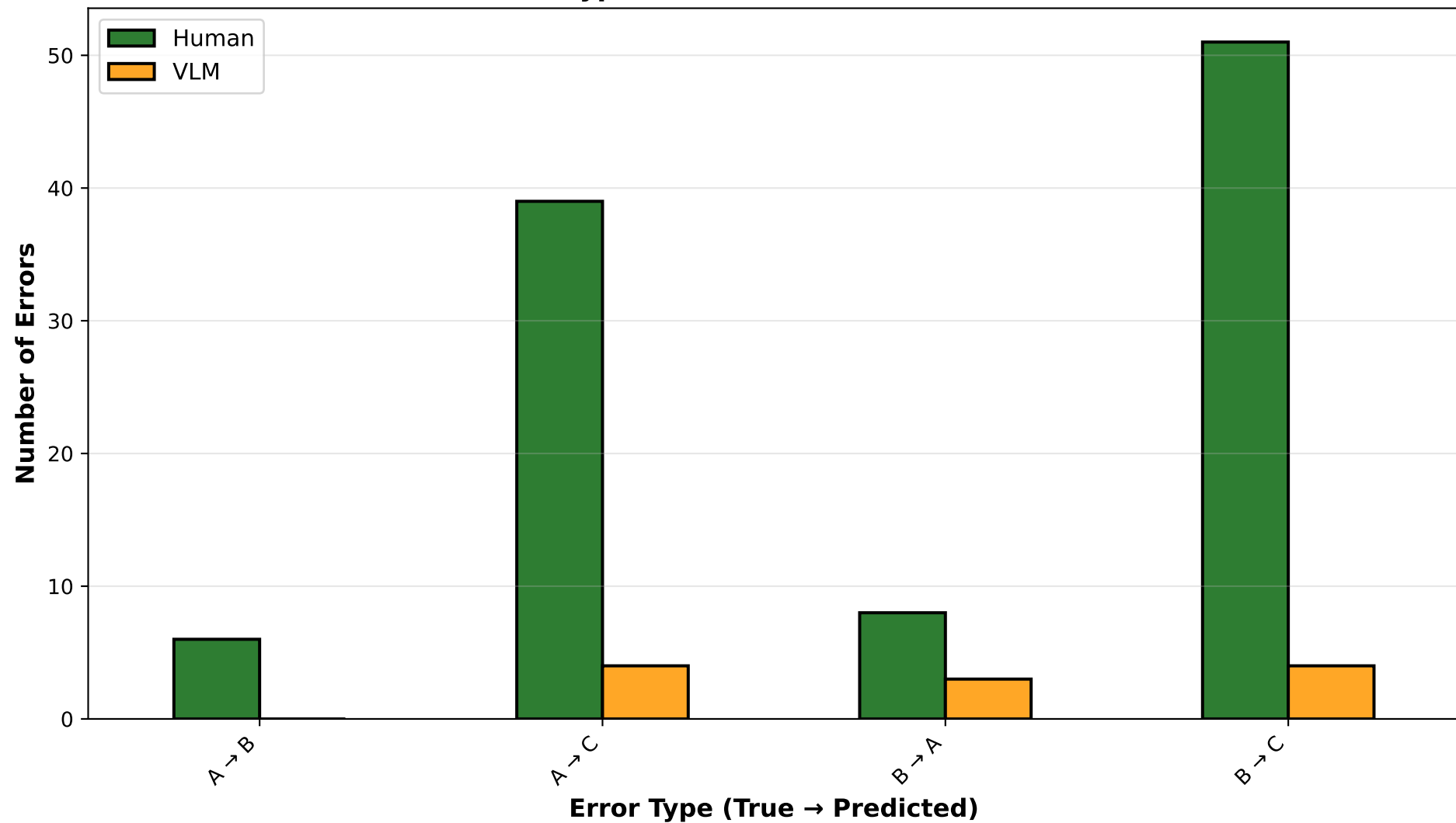
Error Type Distribution: Human vs VLM
