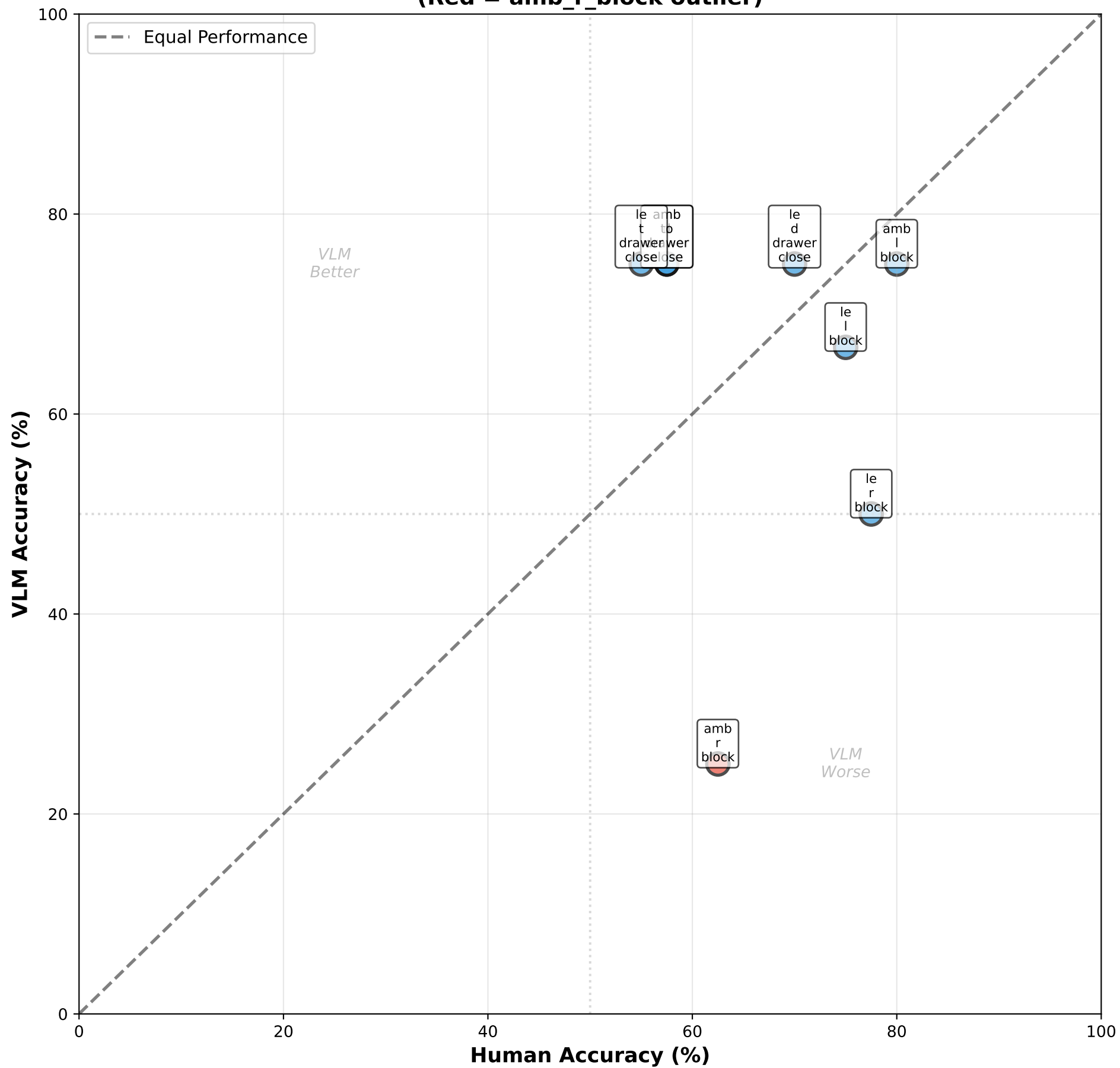
Human vs VLM Accuracy Per Video (Red = amb_r_block outlier)
