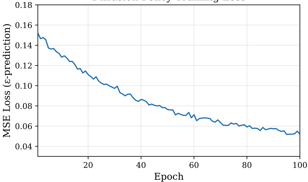
Diffusion Policy Training Loss
