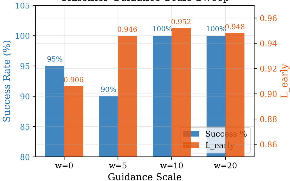
Classifier Guidance Scale Sweep
