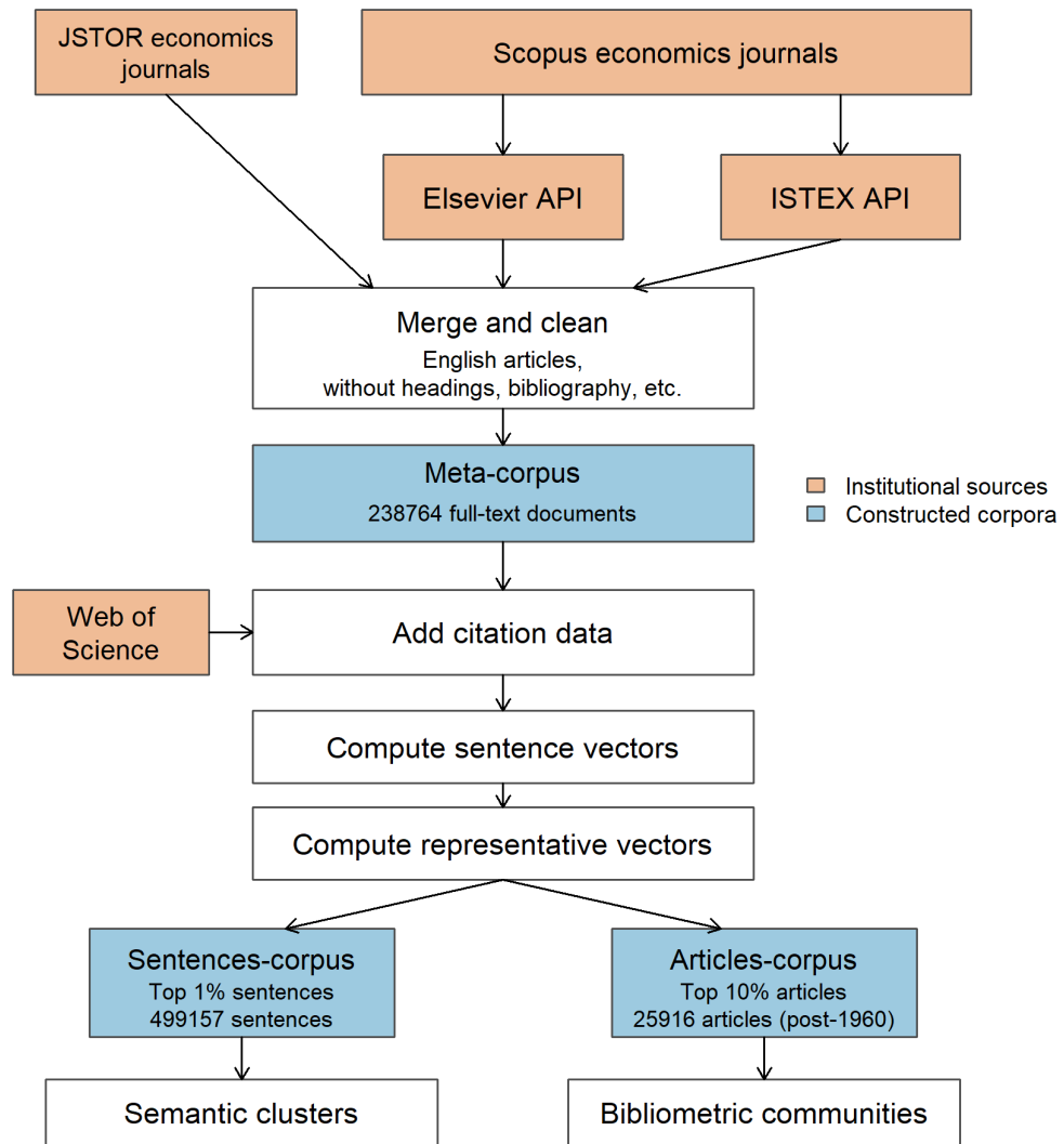
Figure 1.: General workflow of the methods used in the paper. Orange boxes represent data sources. Blue boxes represent used corpora. White boxes are transformation steps. Arrows indicate the flow of data and transformations.
