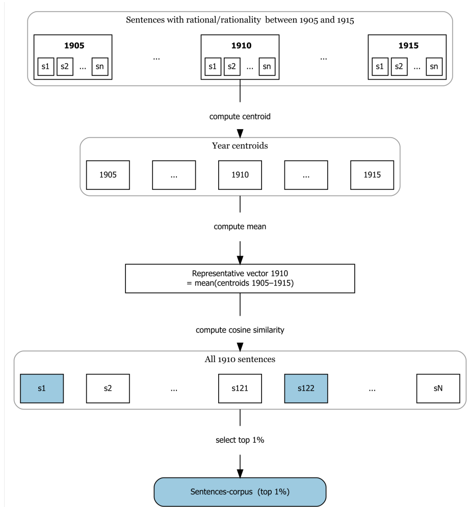
Figure 2.: Zoom on the construction of the representative vector of rationality and how it is used to build a corpus (here the sentences-corpus). White boxes are transformation steps. Arrows indicate the flow of data and transformations.
