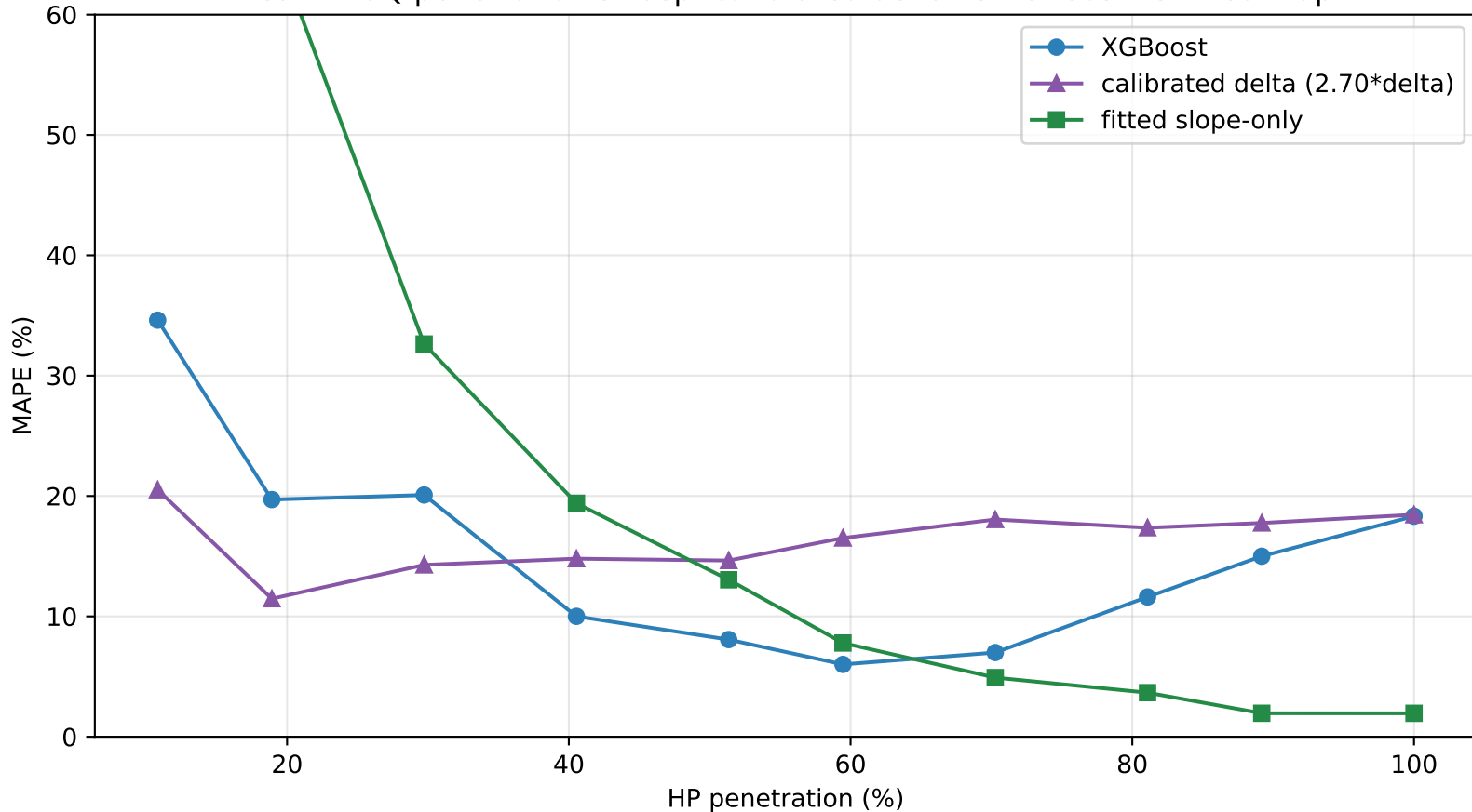
Real WPUQ penetration sweep: calibrated delta vs XGBoost vs fitted map
