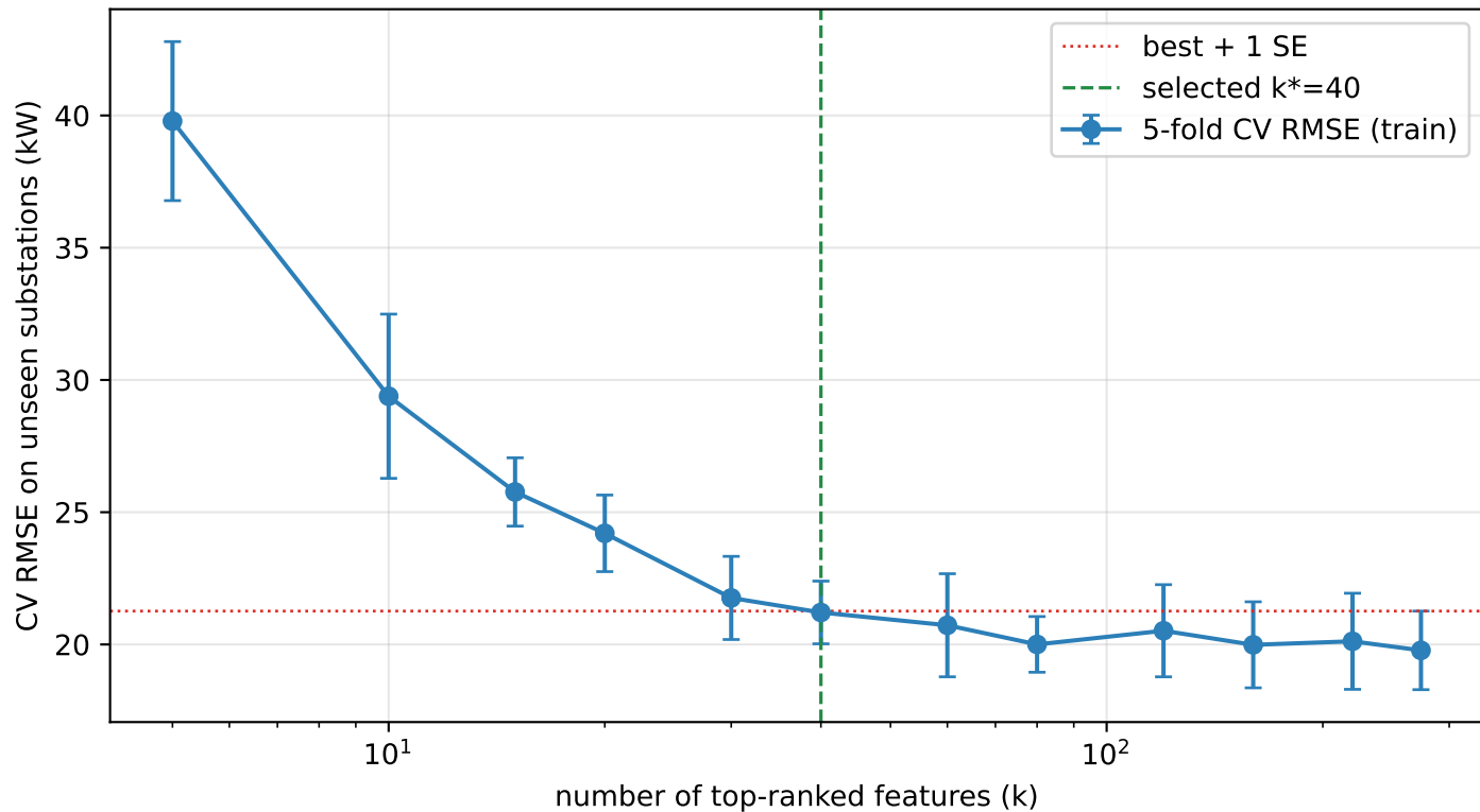
XGBoost feature selection -- CV error vs feature-set size
