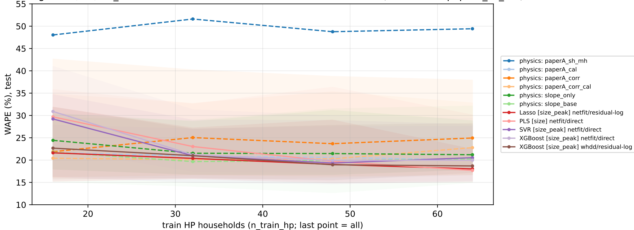
Learning curve, B^* , HP_Peak: median and 5%-90% band over seeds x draws (no band for paperA_sh_mh)
