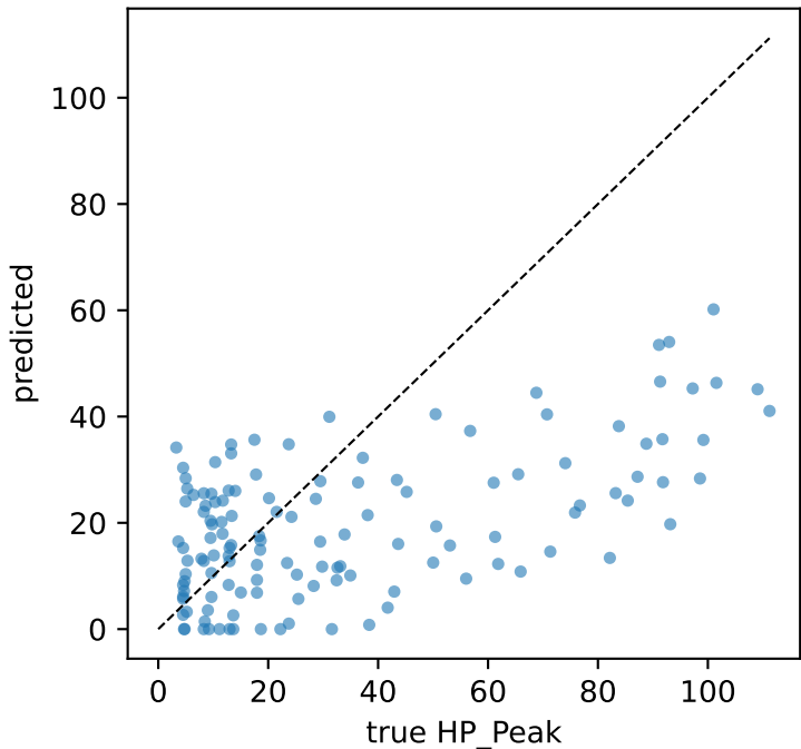
FFNN [size_peak] (test, not interpreted)
