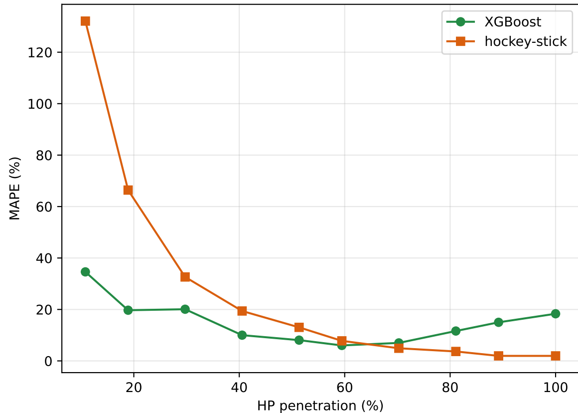
Error vs penetration
