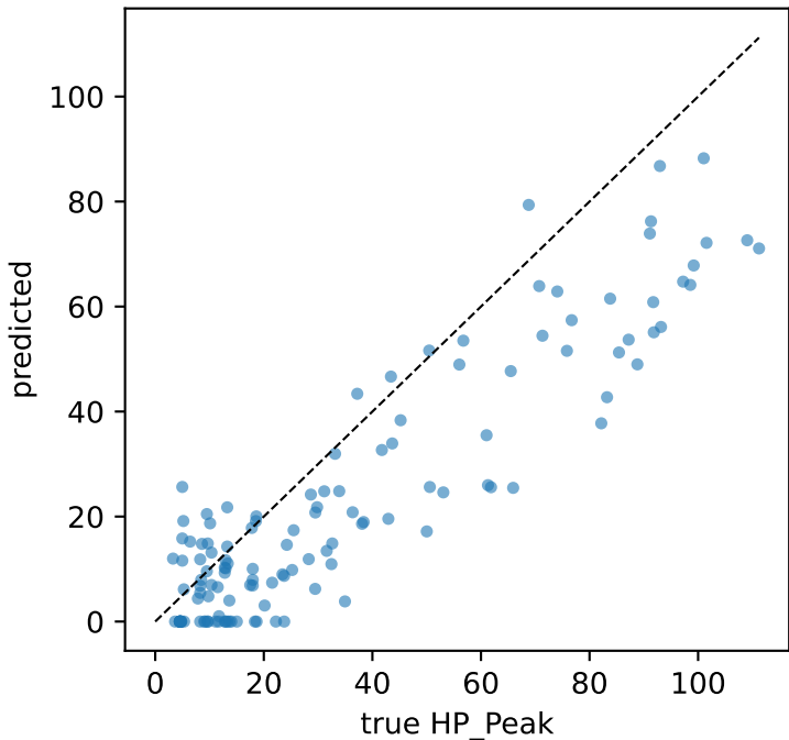
FFNN [none] (test, not interpreted)
