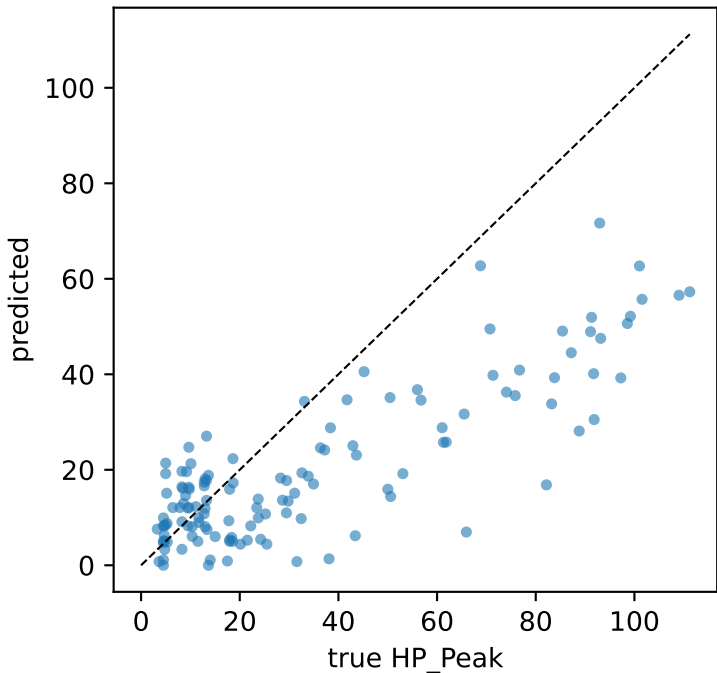
SVR [none] (test, not interpreted)
