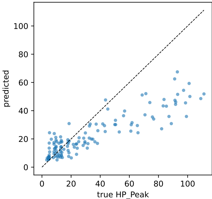
XGBoost [size] (test, not interpreted)
