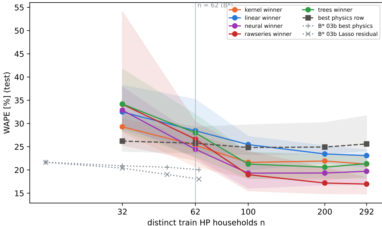
GB dataset, learning curve (overall)
