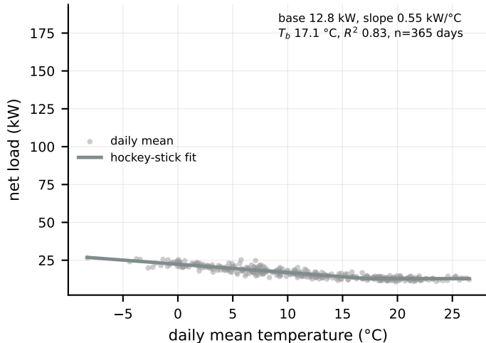
0 % heat pump penetration (48 consumers)
