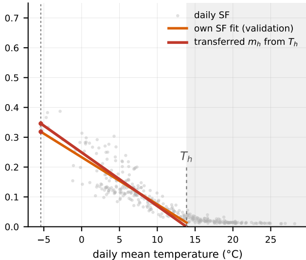
simultaneity factor SF
