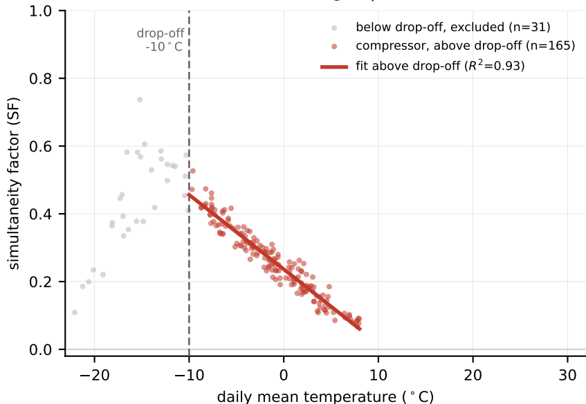
Hennepin MN ResStock ASHP -- SF, compressor-only below -10^{\circ}\text{C} excluded, \text{SF@dropoff}=0.46 , R^2=0.93
