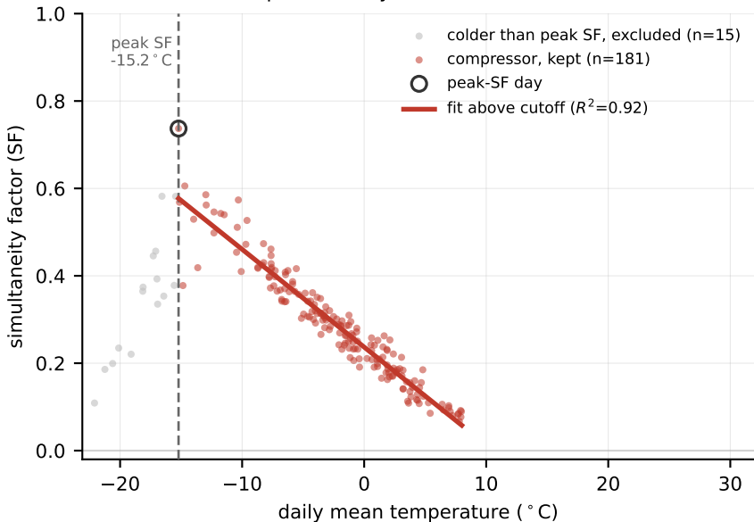
Hennepin MN ResStock ASHP -- SF, compressor-only colder than peak-SF day ( -15.2^{\circ}\text{C} ) excluded, R^2=0.92
