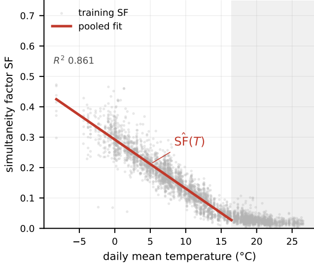
Fig. 7. The single \hat{SF} curve fitted to the pooled daily (T, SF) points of the training substations (grey), used as the transferable curve, at an R^2 of 0.861.
