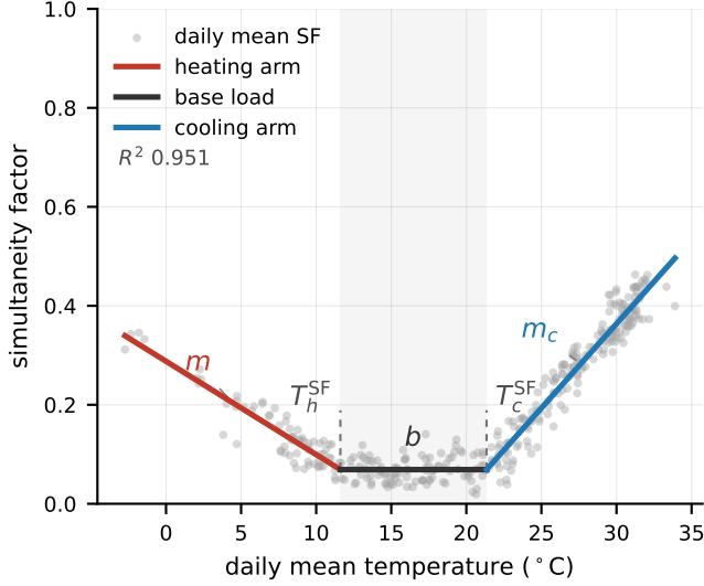
Fig. 3. Equation (7) fitted to the SF of the aggregated Austin ETLs [?], with each daily point normalised by the installed capacity of the ETLs active in its regime (Equation (6)).
