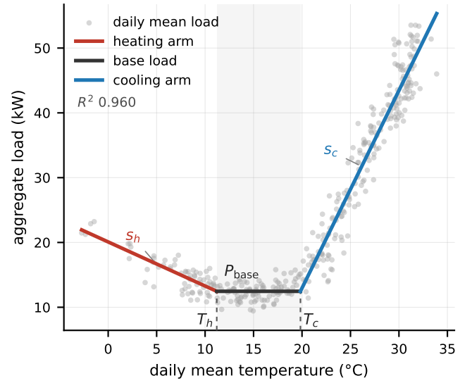
Fig. 2. Equation (2) fitted to daily mean load of an aggregation of air-conditioned and furnace-heated dwellings in Austin, Texas [?].
