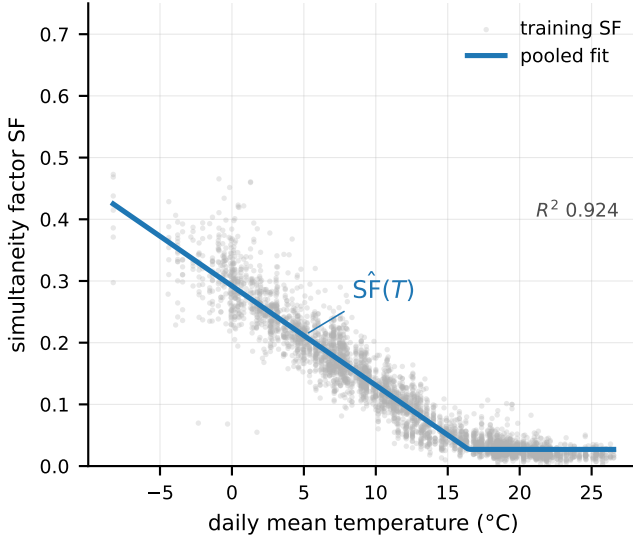
Fig. 7. The single SF curve fitted to the pooled daily (T, SF) points of the training substations (grey), used as the transferable curve, at an R^2 of 0.92.
